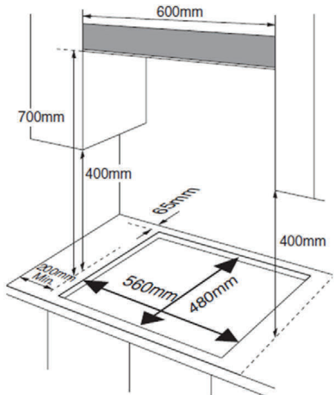
Required distances when installing the panel under the kitchen hood
